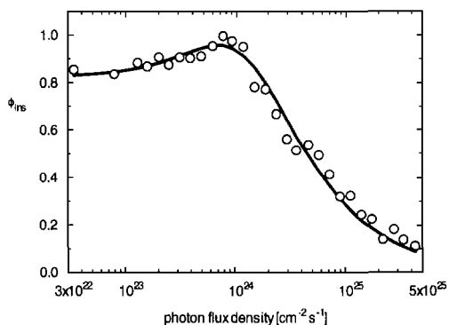
Fig. 5. \phi_{\text{ins}} as a “fingerprint” for the excited-state absorption in t_4 -PcMg in ethanol. Excitation wavelength, 676 nm; emission wavelength, 730 nm. (○) Data points from the experiment [ \phi_{\text{ins}} was calculated from \varphi_{\text{ins}} and \ln T_2 according to Eq. (7)] and (—) after numerical curve fitting [optimal fit for \sigma_{\text{exc}} (676 nm) = 2.7 \times 10^{-16} \text{ cm}^2 ].
